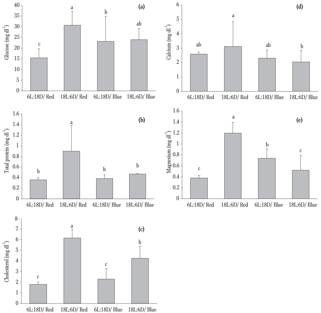
Figure 1. Mean values ( \pm SD) of selected coelomic fluid parameters: glucose (a), total protein (b), cholesterol (c), calcium (d), and magnesium (e) of female starlet ( A. ruthenus ) broodstocks reared under different colored light and photoperiod treatments.
